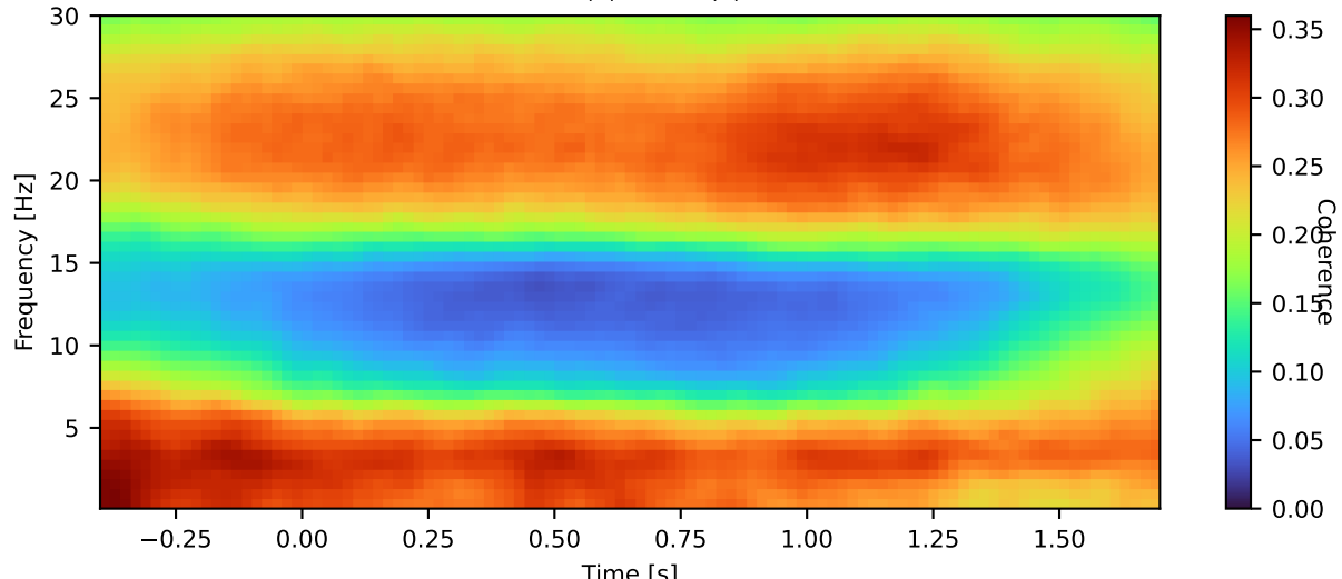
dPFC (6) - dPFC (7)
